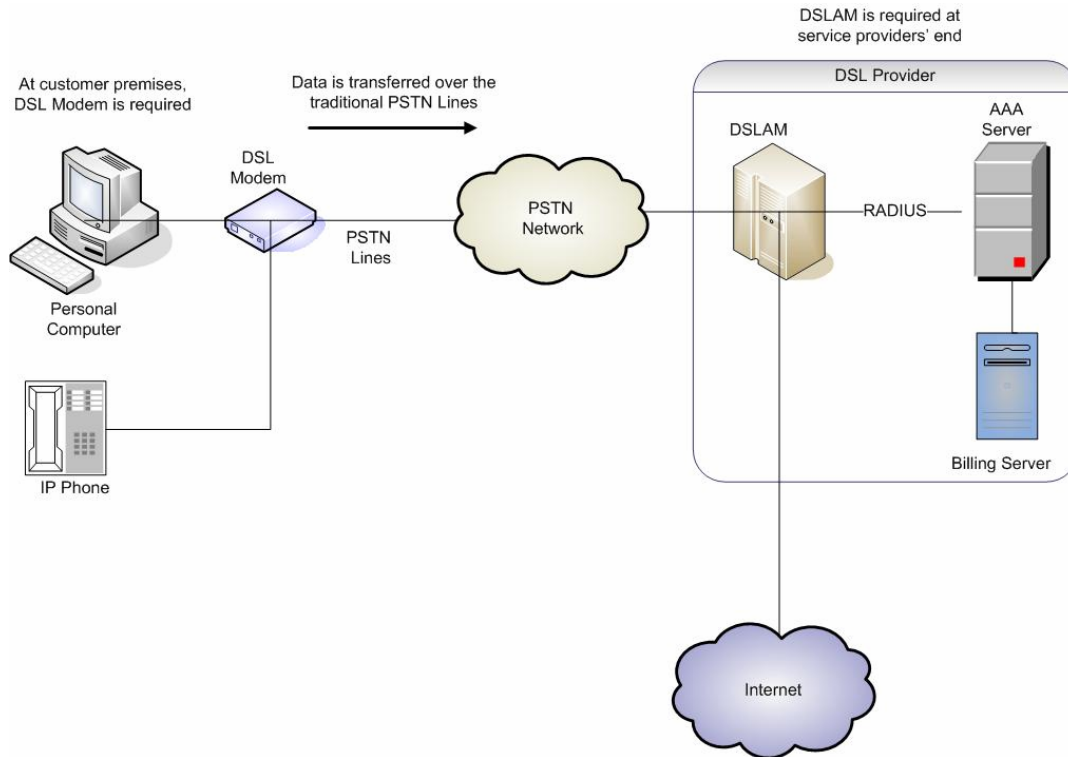
Figure 01: DSL Setup
